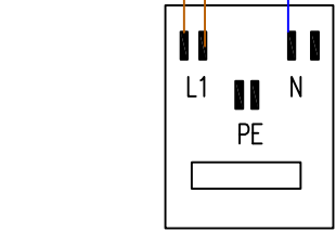
TERMINAL BOX
